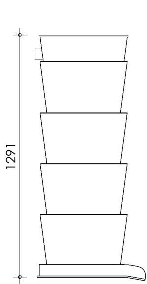
Left-side view
